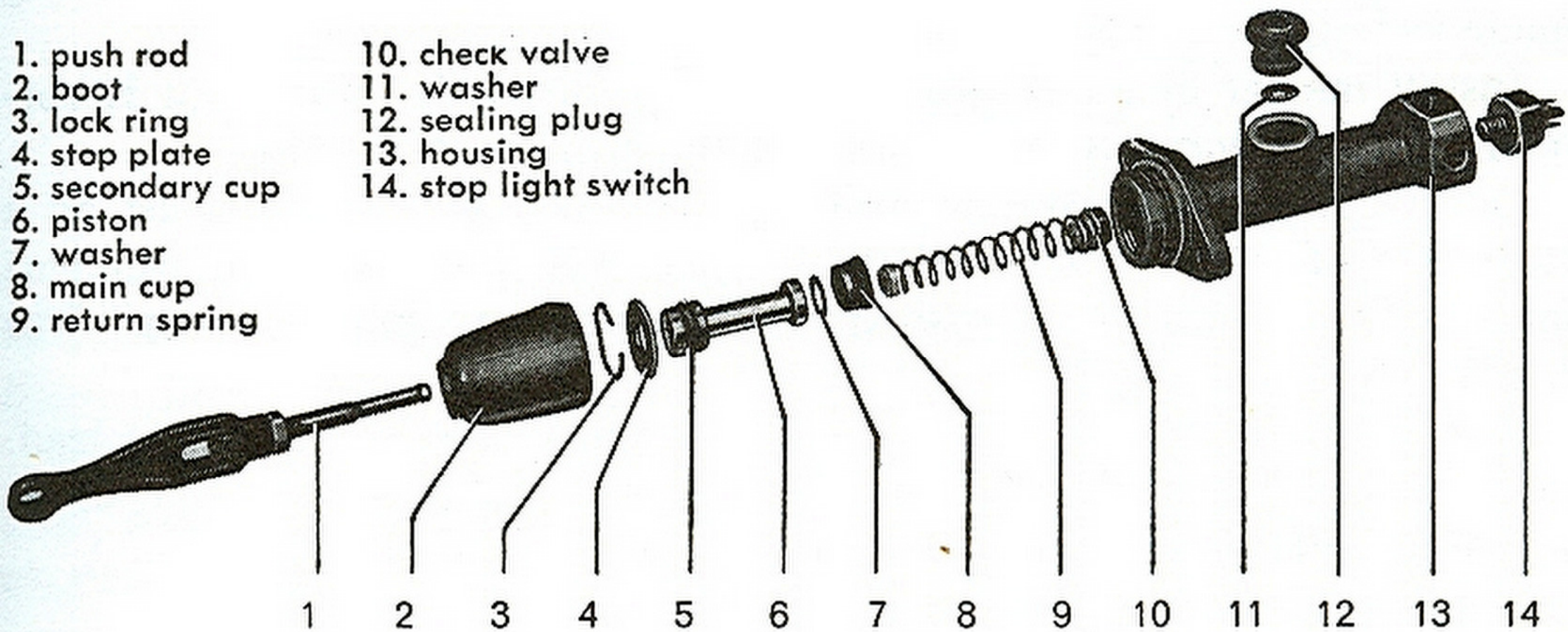
Exploded view of brake master cylinder for single circuit brakes
